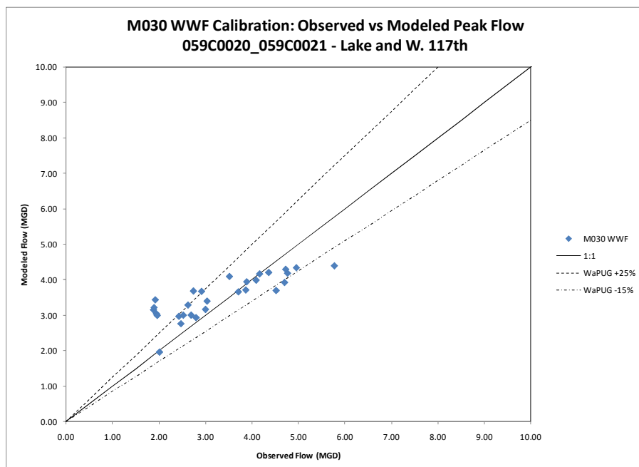
Figure 6.52: M030 WWF Flow Calibration Plot
