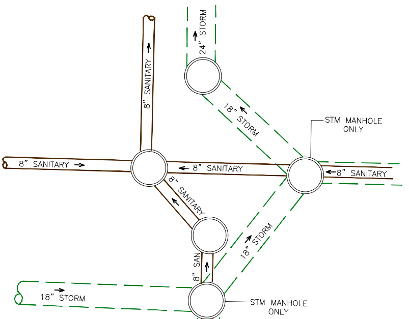
DETAIL ELBUR AND MERL N.T.S.
