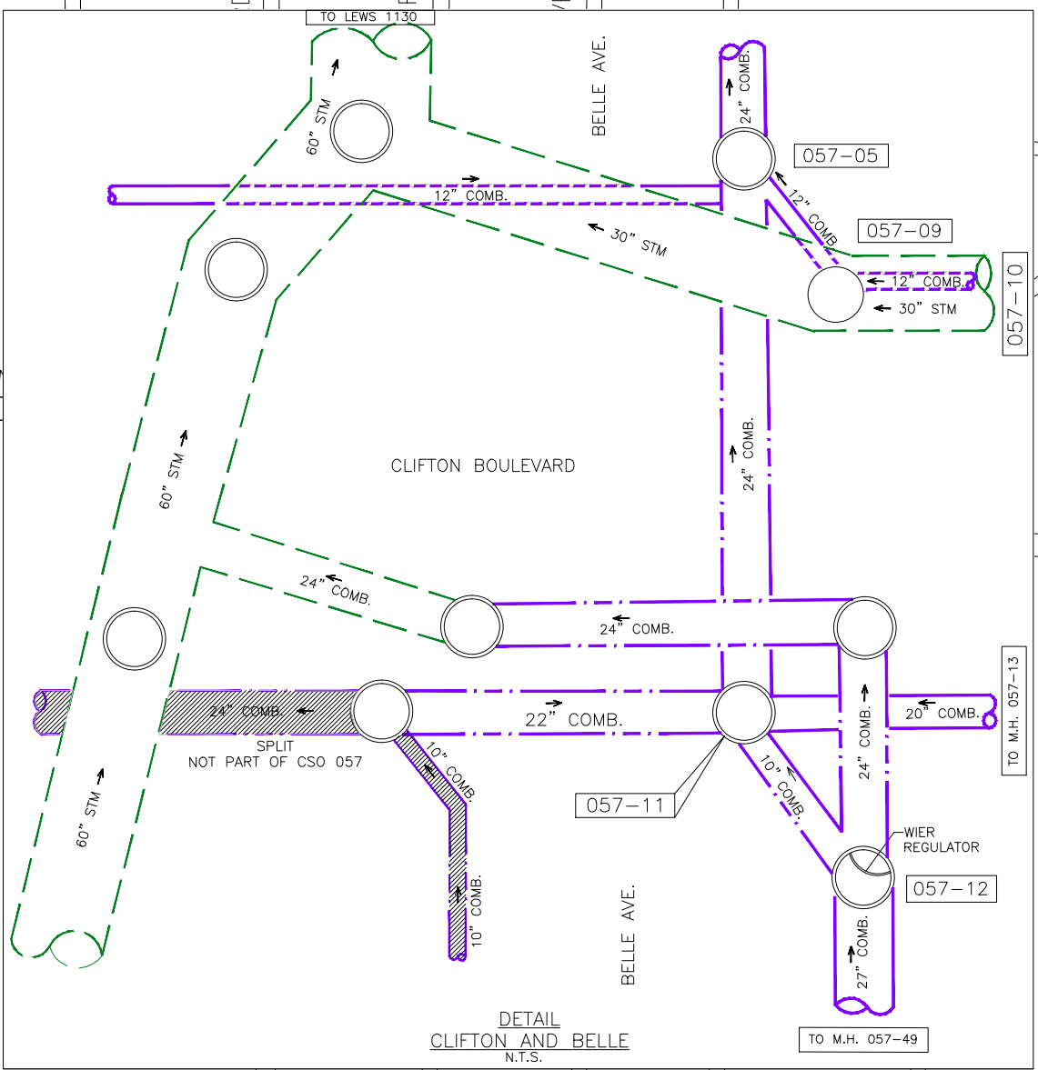
DETAIL CLIFTON AND BELLE N.T.S.
