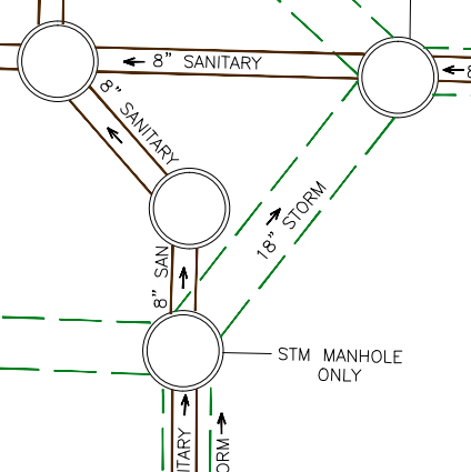
DETAIL ELBUR AND MERL N.T.S.
