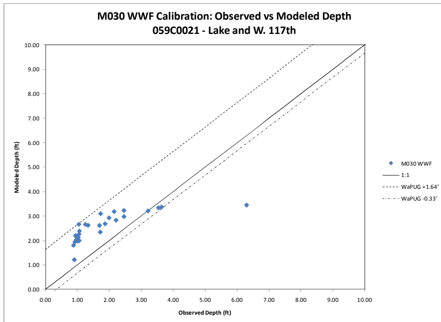
Figure 6.51: M030 WWF Depth Calibration Plot
