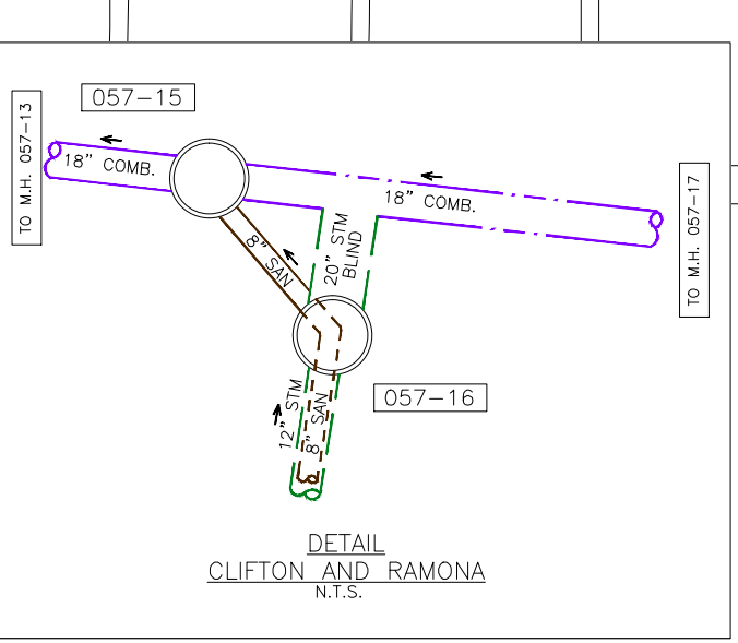
DETAIL CLIFTON AND RAMONA N.T.S.
